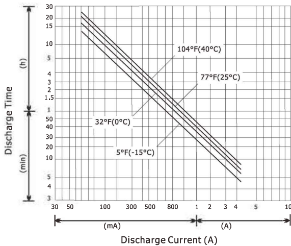
Discharge Curves 77°F(25°C)
